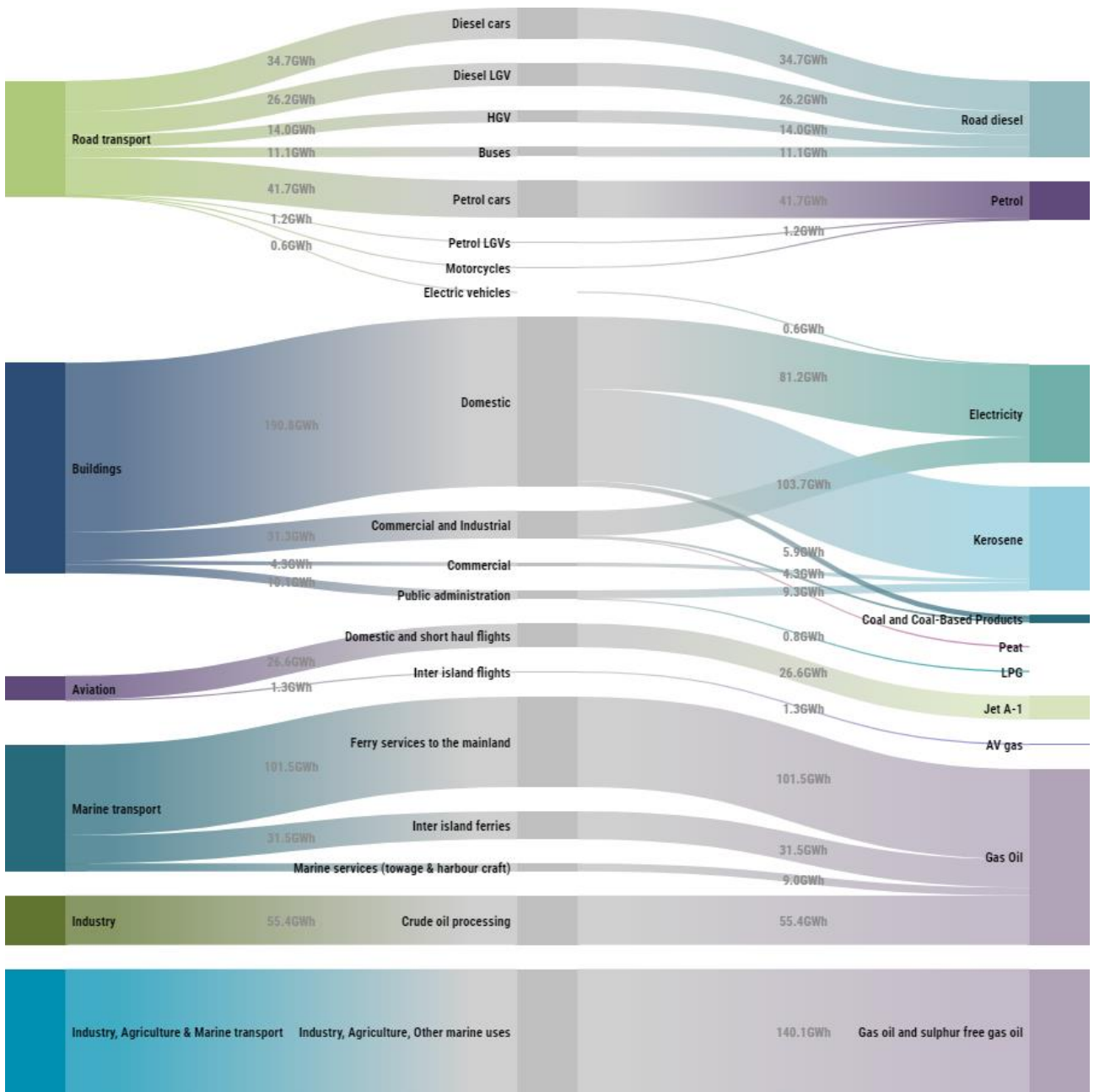
Figure 1 Sankey diagram showing Orkney's energy use by sector and end use (GWh)
