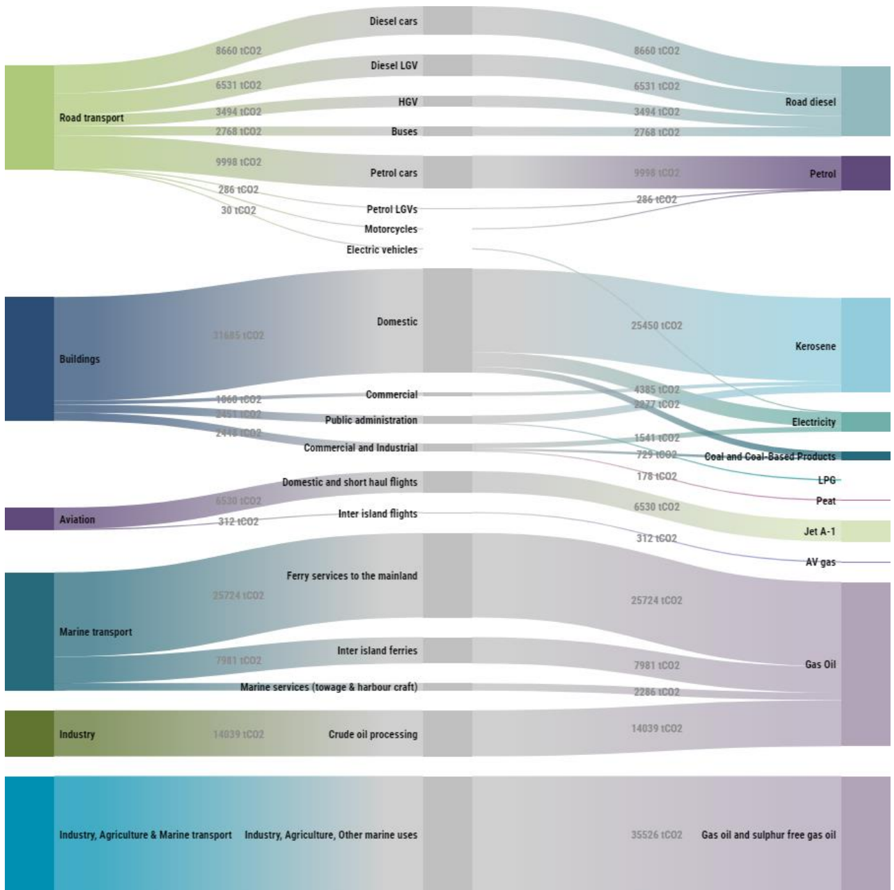
Figure 2 Total annual carbon emissions for Orkney (Tonnes of CO 2 )
